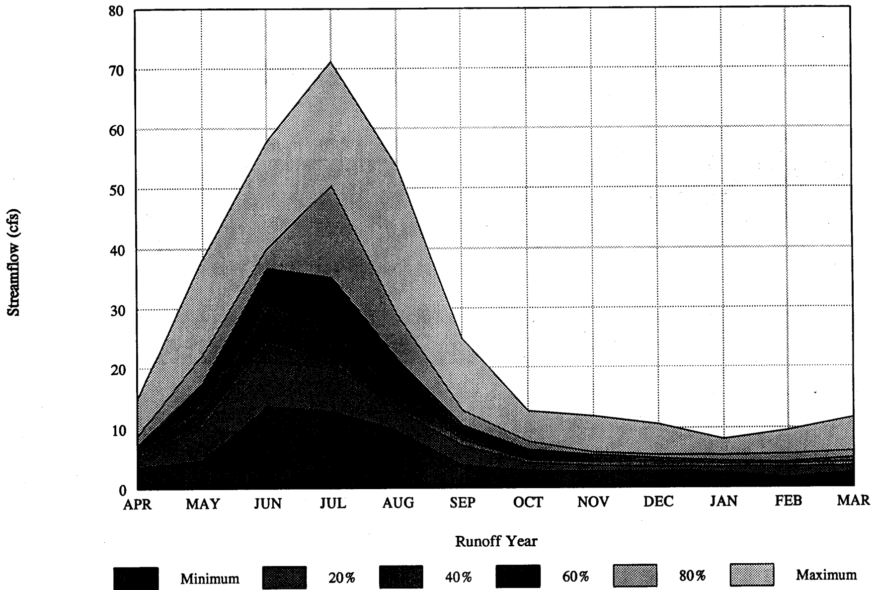
Figure 3A-4. Monthly Parker Creek Streamflow Distribution
