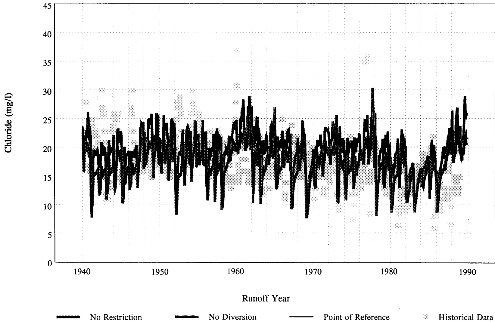
Figure 3B-9. Predicted and Historical Chloride Concentrations for LA Aqueduct Filtration Plant Inflow from 1940 to 1990
