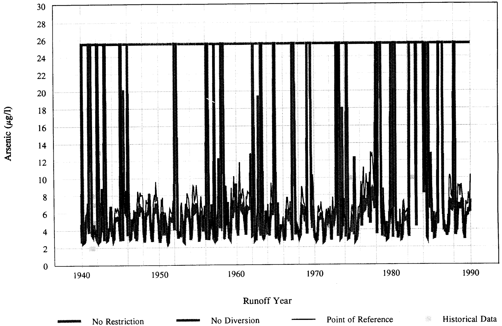
Figure 3B-12. Predicted and Historical Arsenic Concentrations for East Portal Outflow from 1940 to 1990
