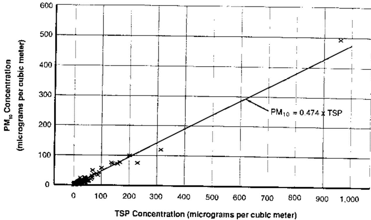
Figure 3H-7. Simis Ranch PM 10 /TSP Relationship, May 1990-June 1992
