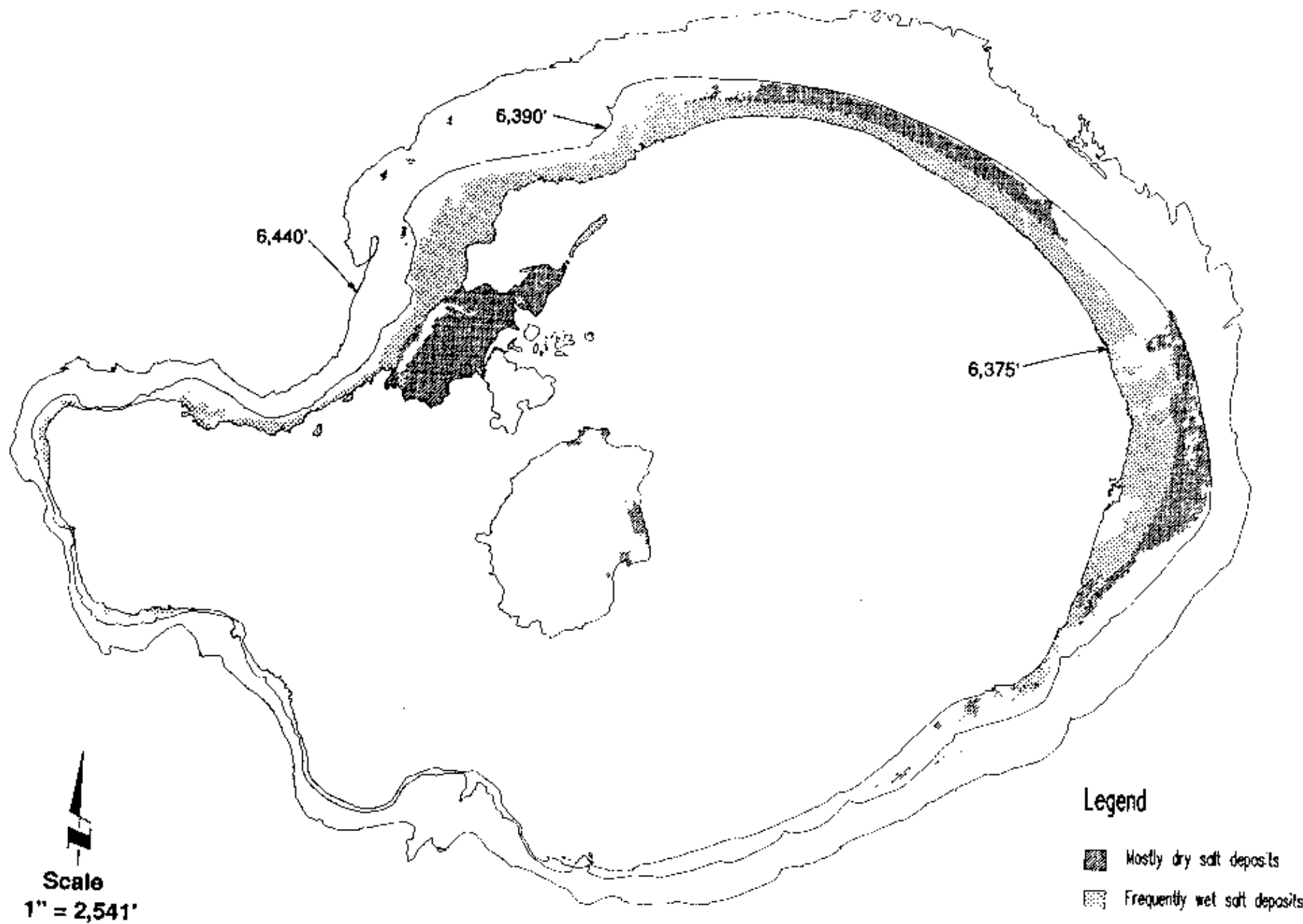
Figure 3H-20. Distribution of Efflorescent Salt Deposits at Mono Lake
