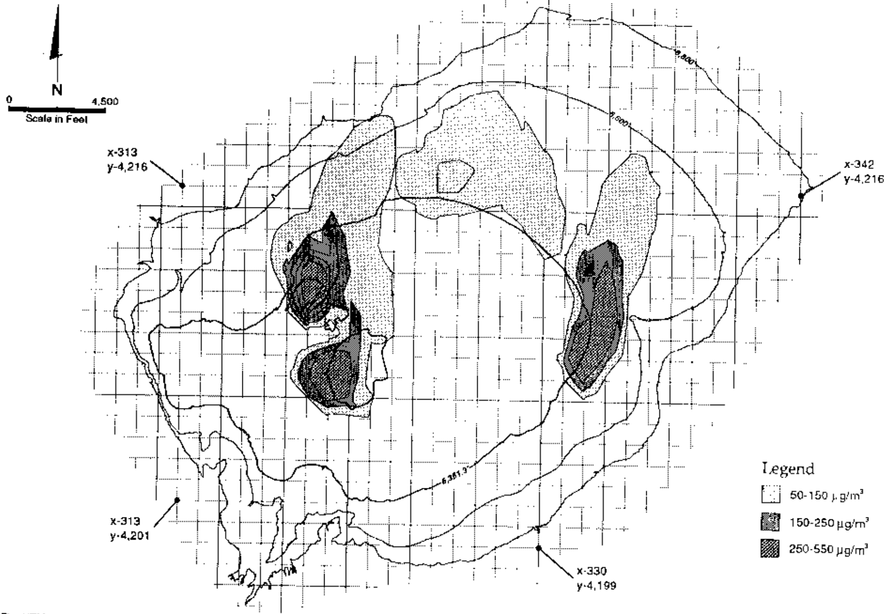
Figure 3H-28. FDM Modeling Results for a Lake Elevation of 6,381.3 Feet on the Maximum Episode Day
